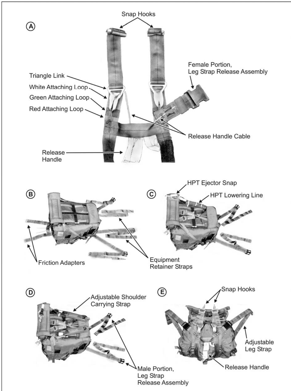
Figure 5-31. Rigging the HSPR
