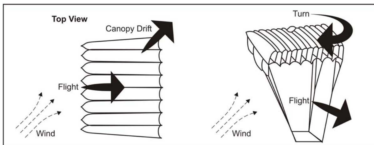
Figure 8-14. Crabbing Maneuver
