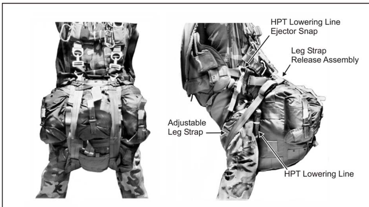
Figure 5-33. Parachutist With HSPR-Rigged Combat Pack
