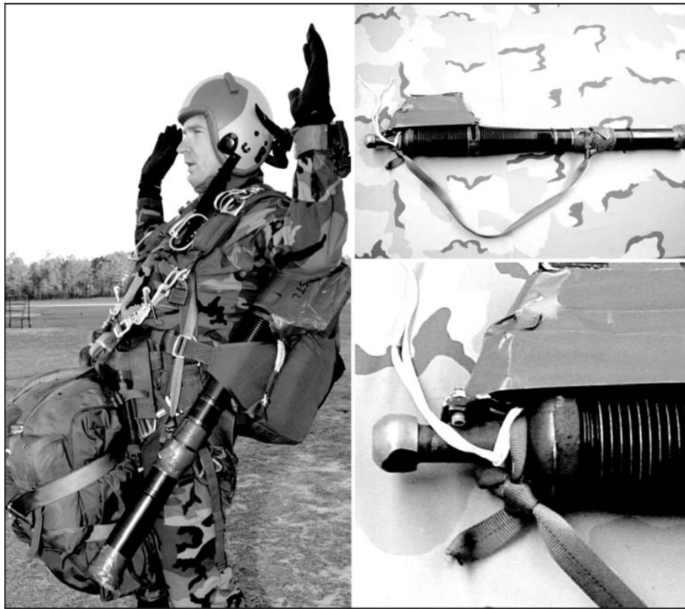
Figure 5-56. Left-Side Mount for M224 60-mm Mortar
