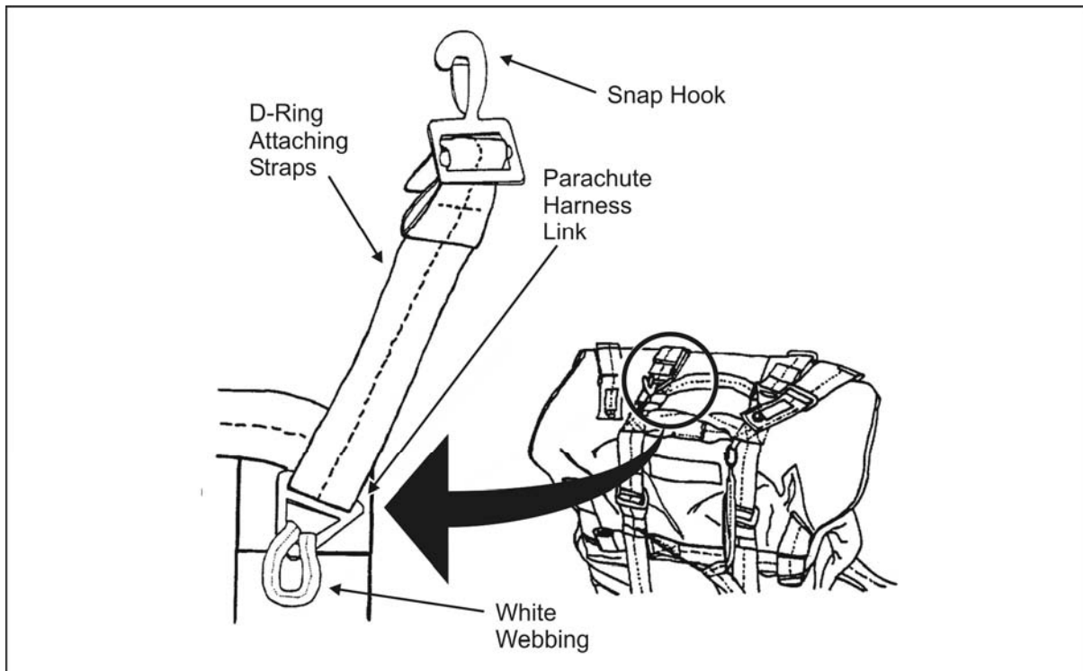
Figure 5-20. Inserting the White Webbing Through the Parachute Harness Link
