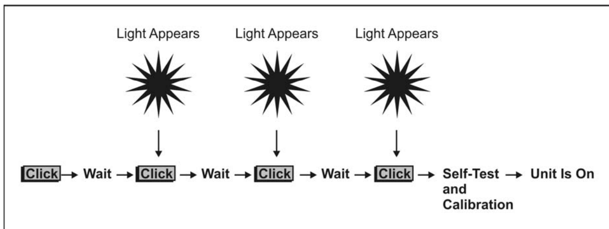
Figure 3-13. Switch-On Procedure
