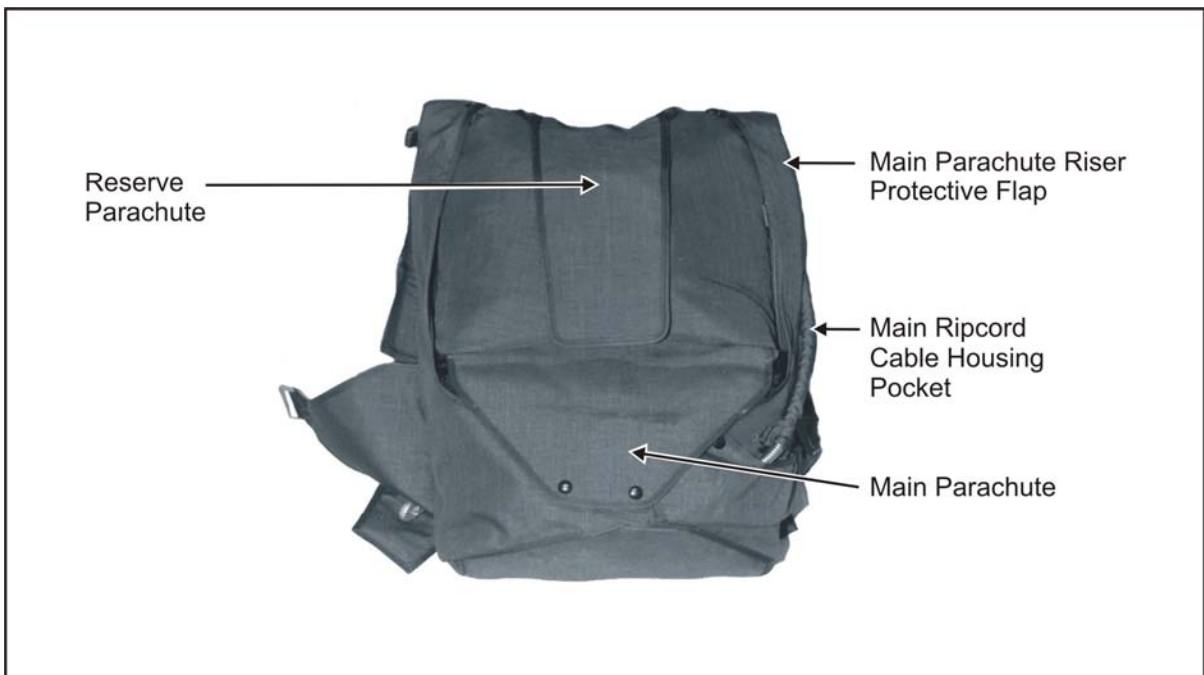
Figure 2-8. Location of the Main and Reserve Parachutes in the Container
