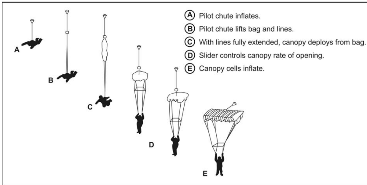
Figure 8-6. Deployment Sequence
