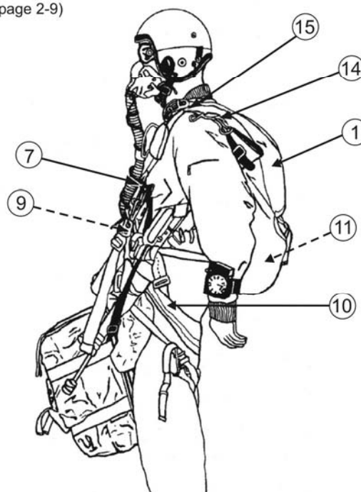
Figure 2-2. MC-4 RAPS Harness and Container Assembly Components
