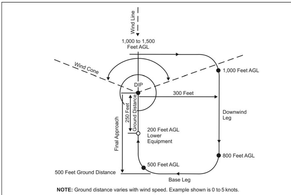
Figure 8-20. Landing Approaches
