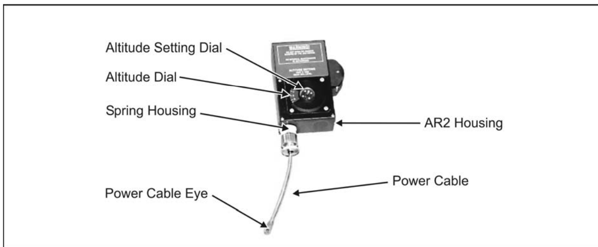
Figure 3-4. AR2 Components
