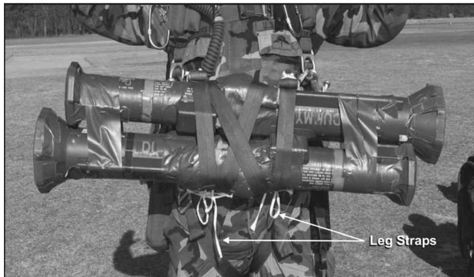
Figure 5-53. Front-Mounted Weapon With Rear-Mounted Rucksack
