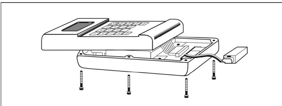
Figure 3-7. Battery Replacement
